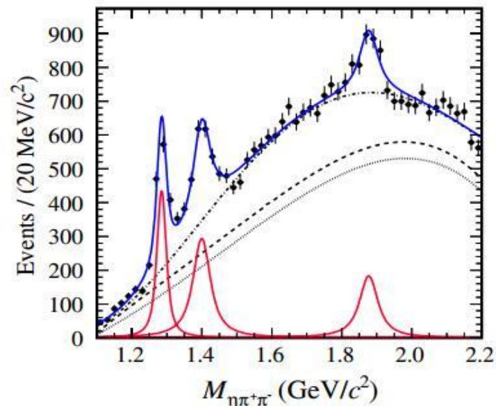
FIG. 4 (color online). Results of the fit to the M(\eta\pi^+\pi^-) mass distribution for events with either the \eta\pi^+ or \eta\pi^- in the a_0(980) mass window. The dotted curve shows the contribution of non- \omega and/or non- a_0(980) background, the dashed line also includes the contribution from J/\psi \rightarrow b_1(1235)a_0(980) , and the dot-dashed curve indicates the total background with the non-resonant J/\psi \rightarrow \omega a_0^\pm(980)\pi^\mp included. \chi^2/\text{d.o.f.} is 1.27 for this fit.
